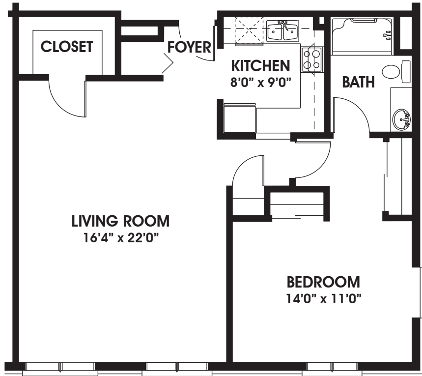
DOROTHY LOVE APARTMENTS ONE BEDROOM DELUXE UNIT 868 S.F.
